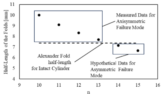
Figure 27: Axisymmetric half-length of fold for ST perforated cylinders ( \theta ).
