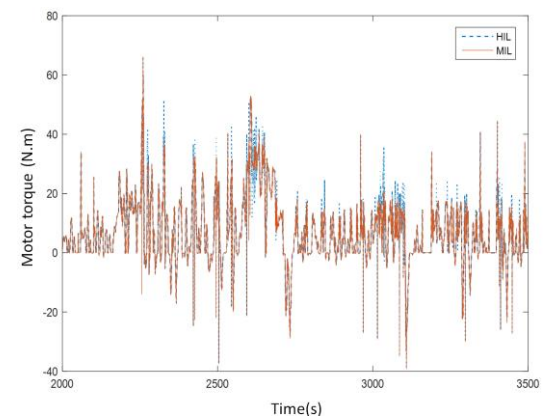
Figure 12: Motor torque (freq. rate: 1000HZ)
