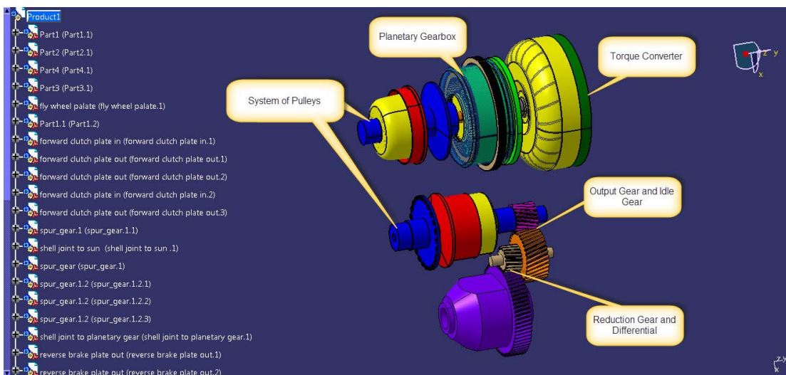
Fig13. : the ultimate mechanism of designed CVT
