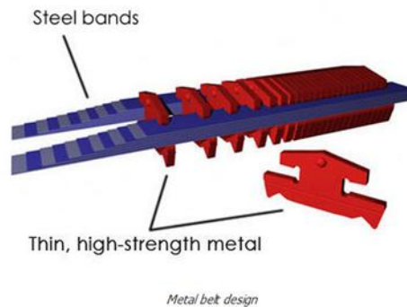
Fig2. steel belt used in pushing belt CVT
